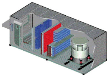
Figure 4: Modular and custom air handlers are ideal products for analysis because they must be able to heat, cool, humidify, and dehumidify air as well as filter particles.
