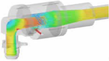
Figure 8: Cyclonic Inertial Separator by David Rachels and engineering team.
