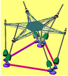
Figure 6: End-of-arm automation tooling designed by Pushcorp, Inc.
