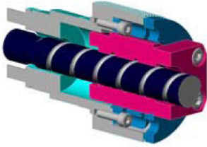
Figure 1: Inner arm of robot designed by Fanuc Robotics
