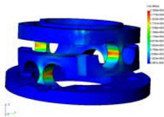
Figure 2: Fanuc Robotics takes full advantage of solid modeler in SolidWorks Simulation.
